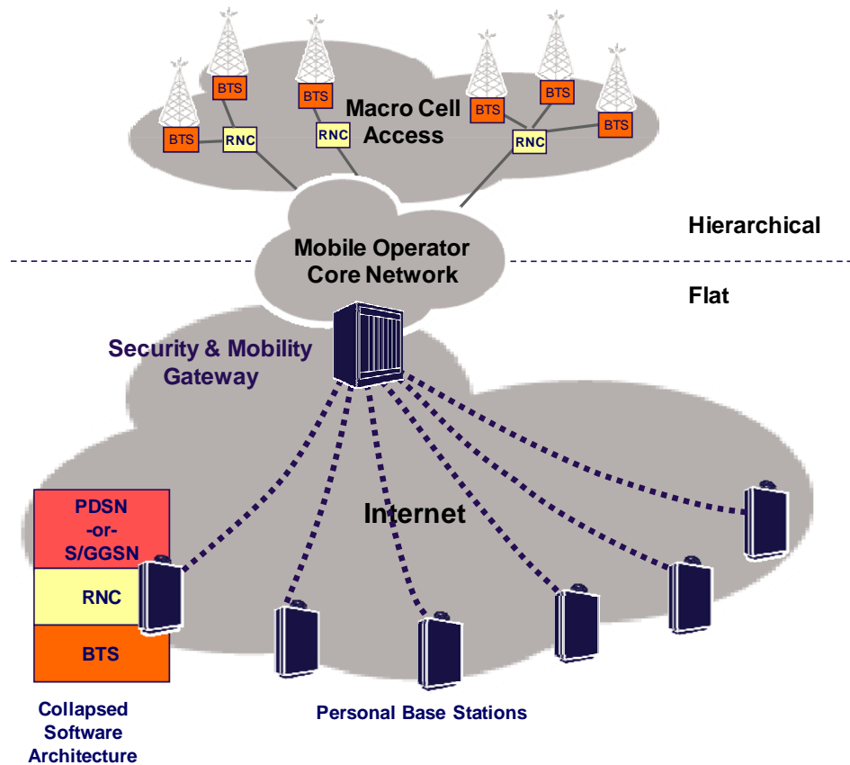
Figure 4: Flat mobile networks of personal base stations
